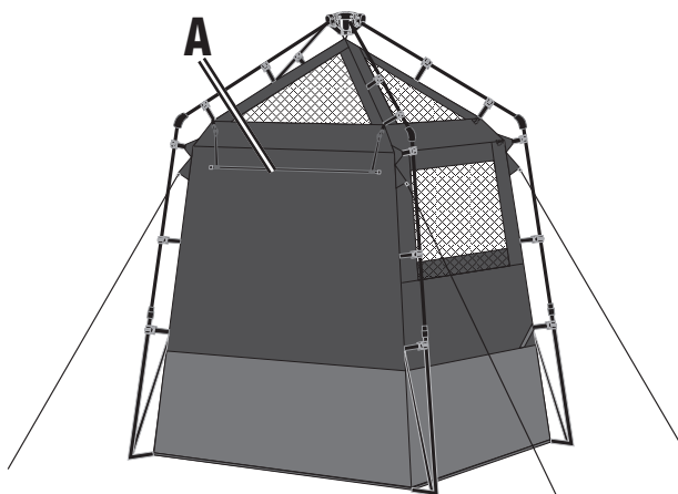
Back view of tent without rainfly
